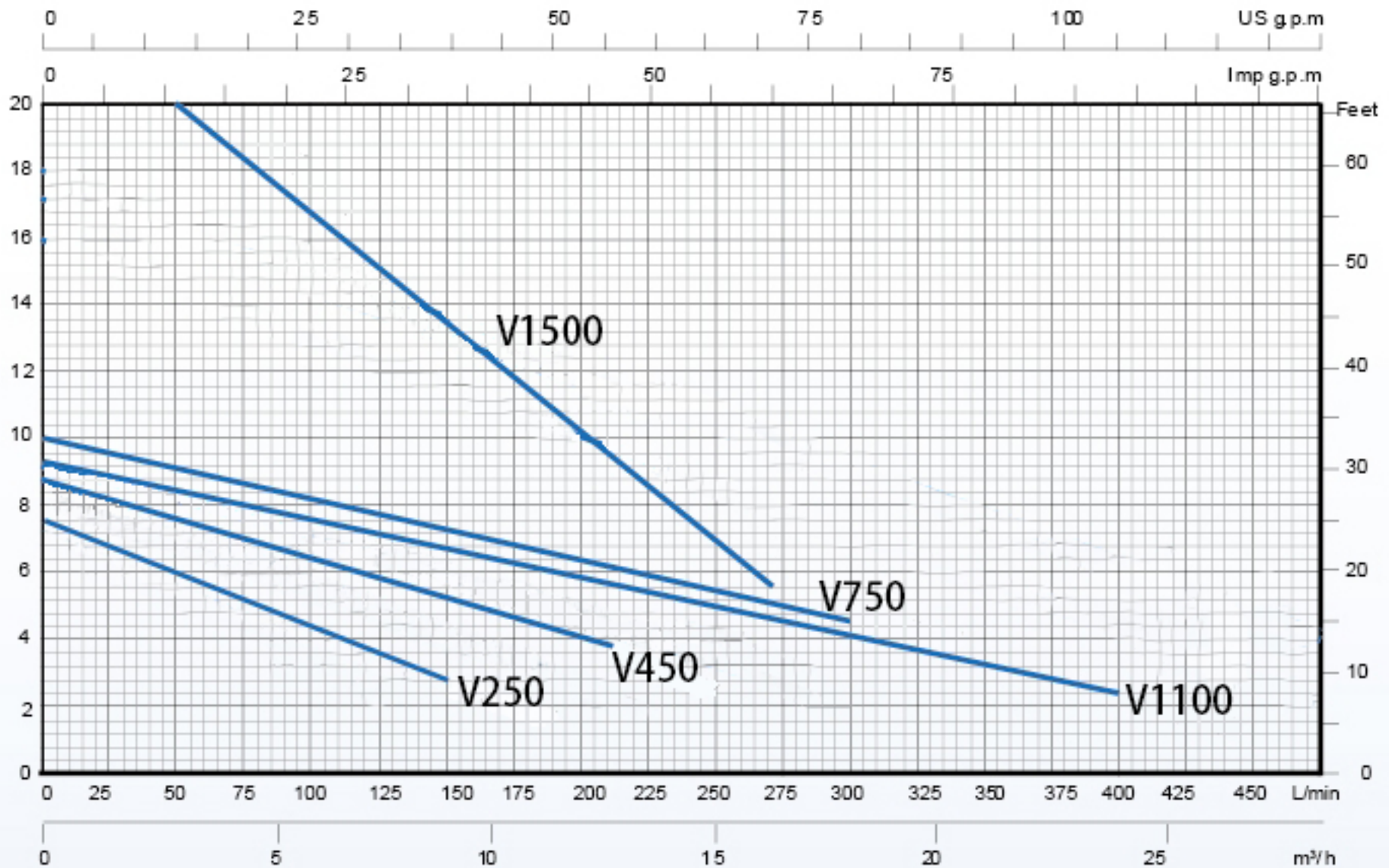
Performance chart at n=2850 r/min(50hz) Total head(m)
